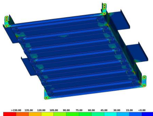
Figure 11, Von Mises Stress on the underside of the platform in [MPa].
